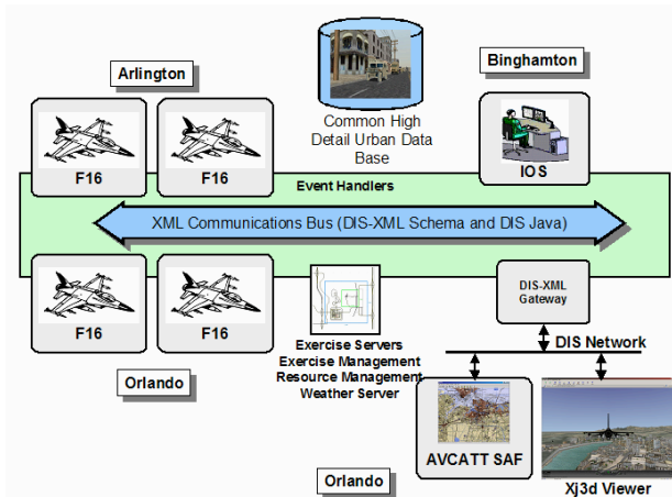
Figure 8. Link Four F16 Ownship Demonstration Configuration
